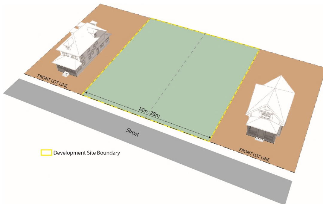
Figure 52. Minimum Street Frontage
