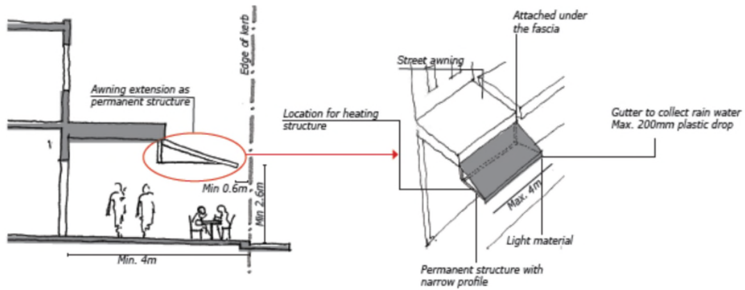
Figure 13. Permanent Awning Extensions
