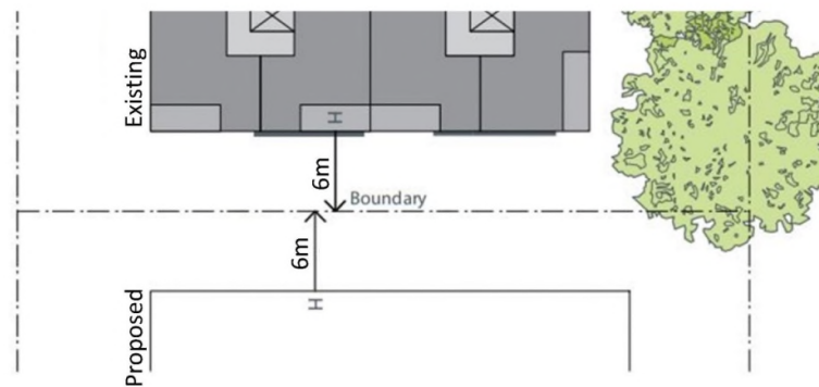
Figure 54. Separation distances
