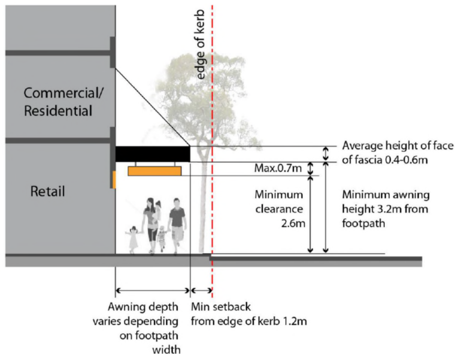
Figure 9. Awning Dimensions
