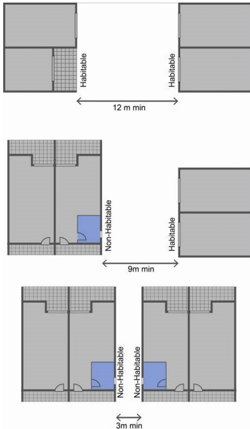
Figure 68. Building Separation for Multi Dwelling Housing
