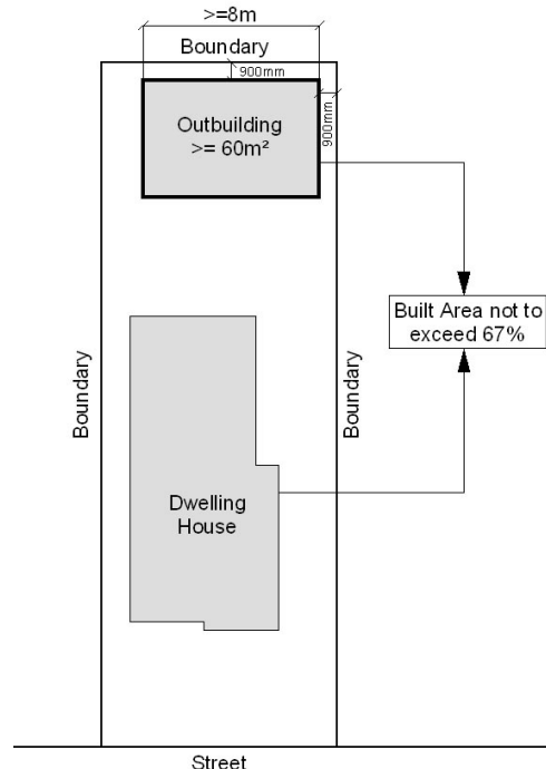
Figure 75. Boundary Setbacks for Substantial Outbuildings
