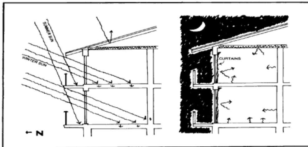
Figure 65. Solar Access and Insulation
